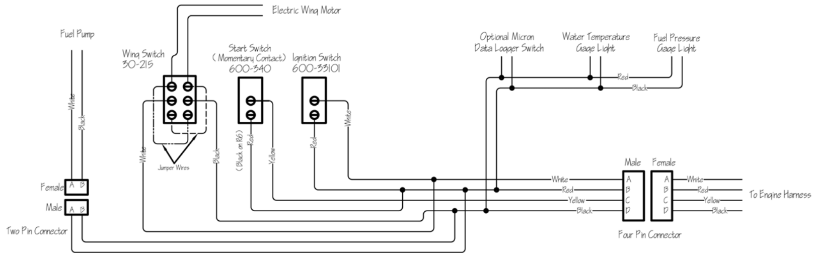
Chassis Harness to Engine Harness Chart
